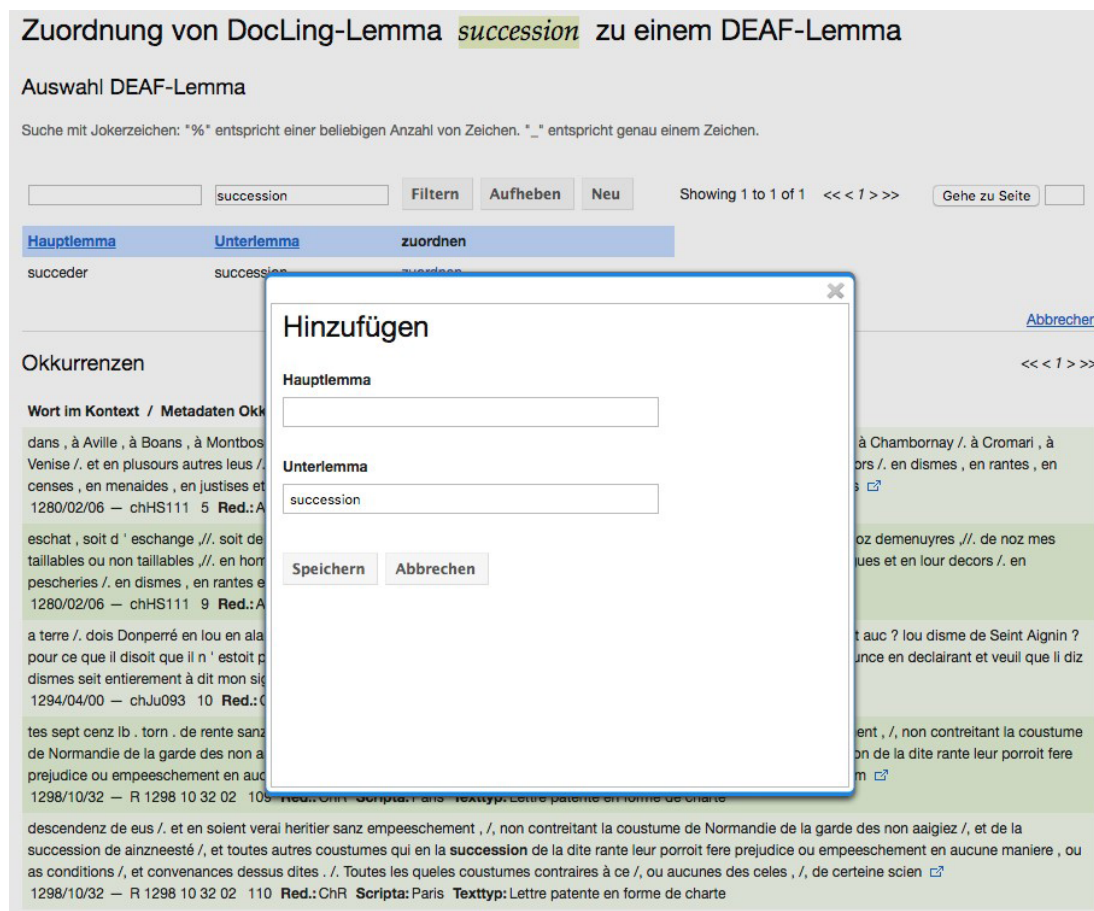
Figure 3: Creation of a new main-lemma-sub-lemma combination.
